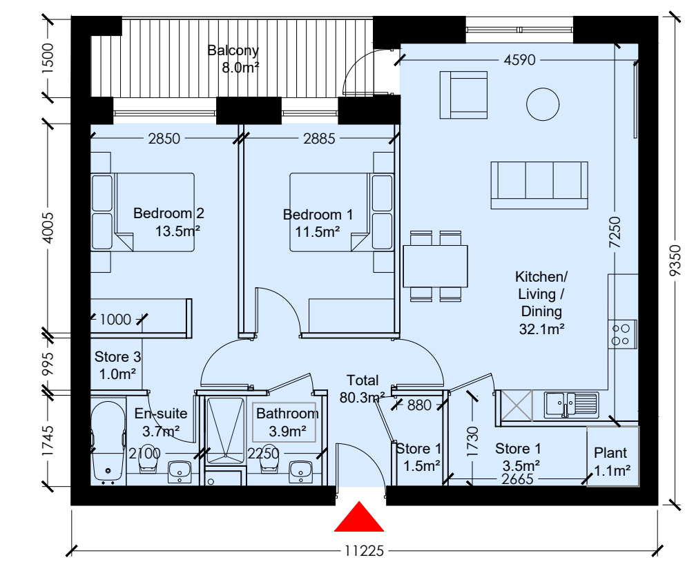
Unit Type 2B_01 Scale 1:100 @ A0
