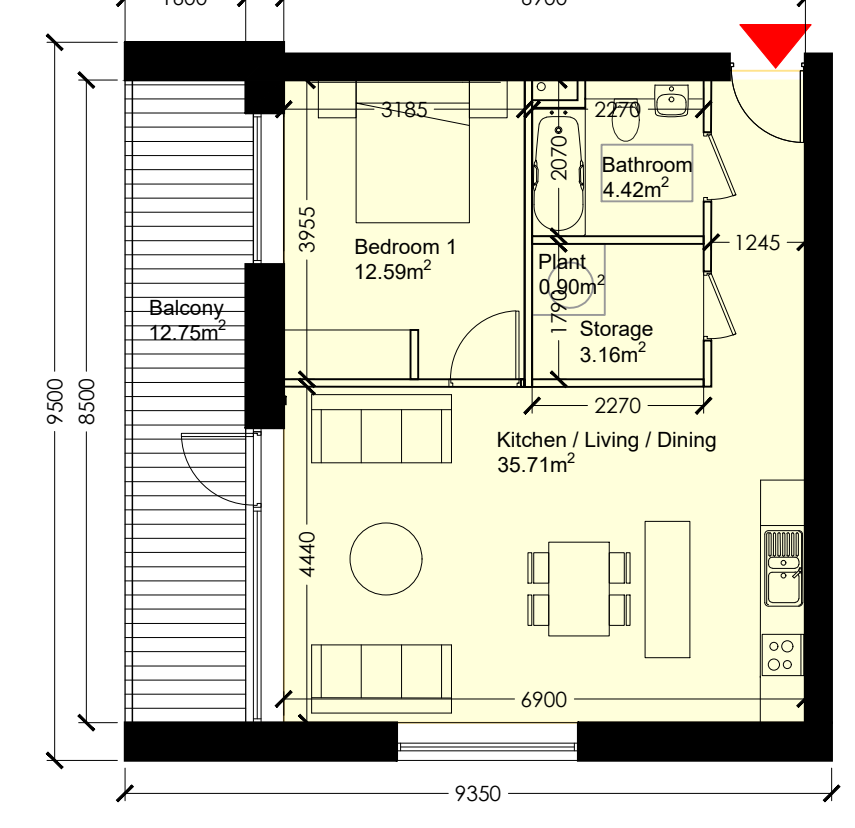
Unit Type 1B_02 Scale 1:100 @ A0
