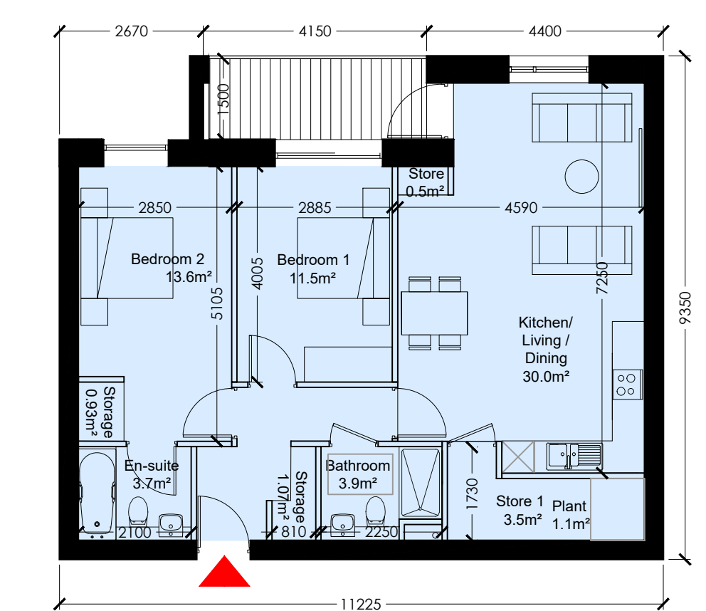
Unit Type 2B_10 Scale 1:100 @ A0
