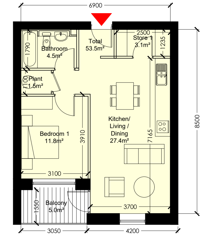
Unit Type 1B_03 Scale 1:100 @ A0
