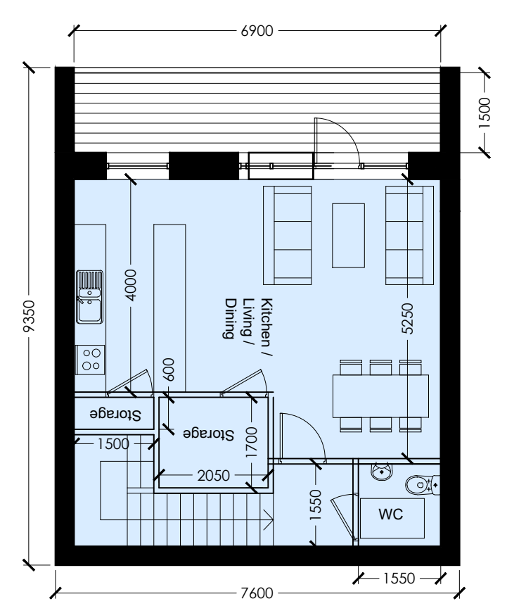
First Floor Level - 47.61 m²
