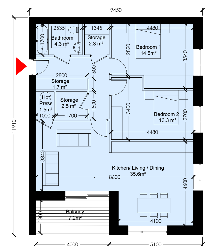
Unit Type 2B_09 Scale 1:100 @ A0
