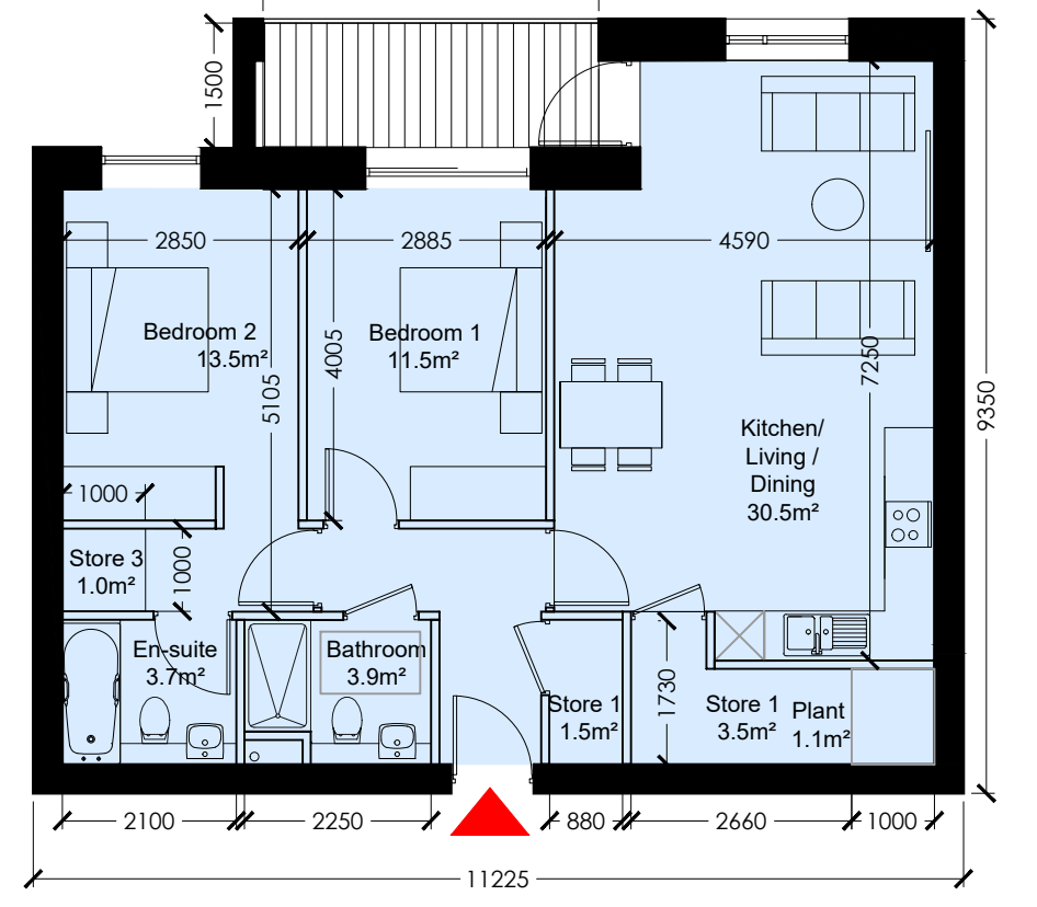
Unit Type 2B_04 Scale 1:100 @ A0
