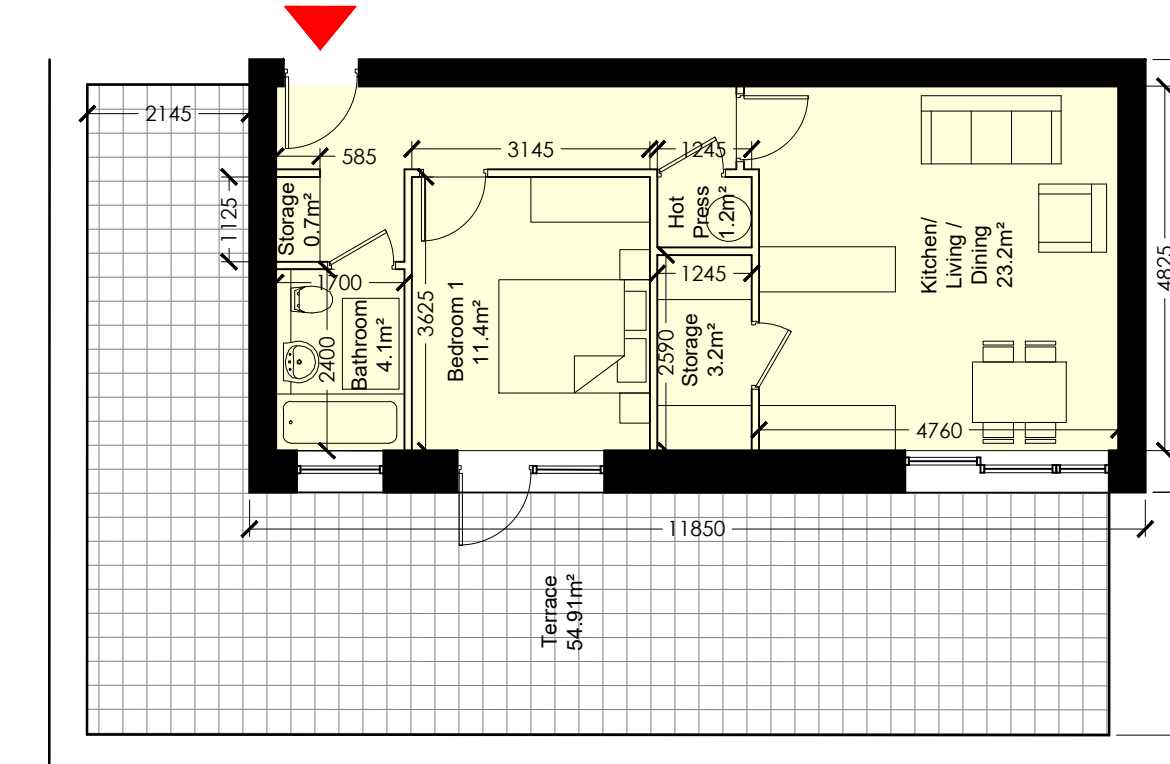
Unit Type 1B_04 Scale 1:100 @ A0
