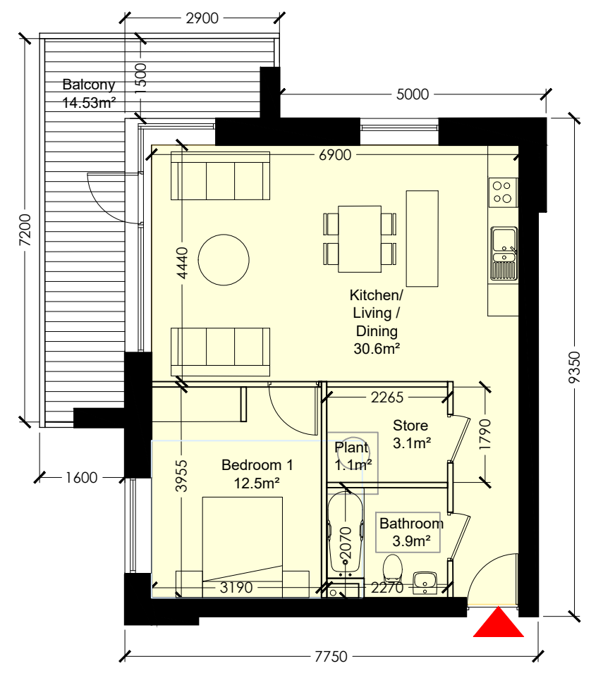
Unit Type 1B_01 Scale 1:100 @ A0
