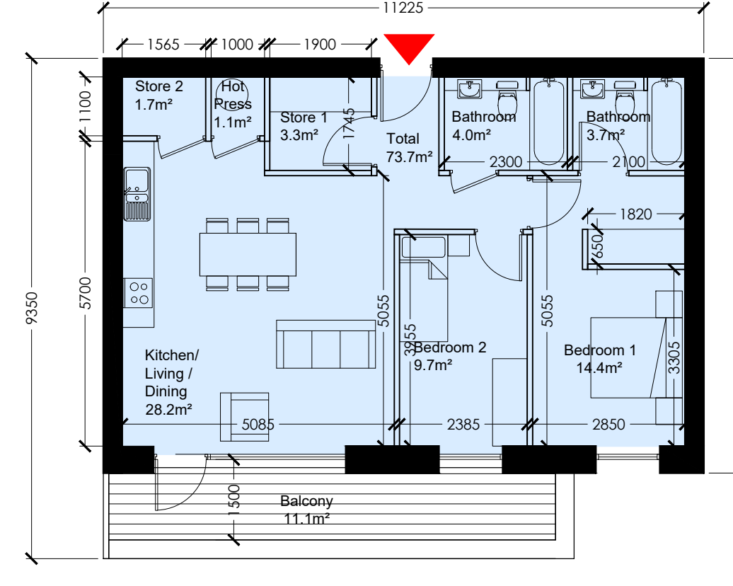
Unit Type 2B_05 Scale 1:100 @ A0
